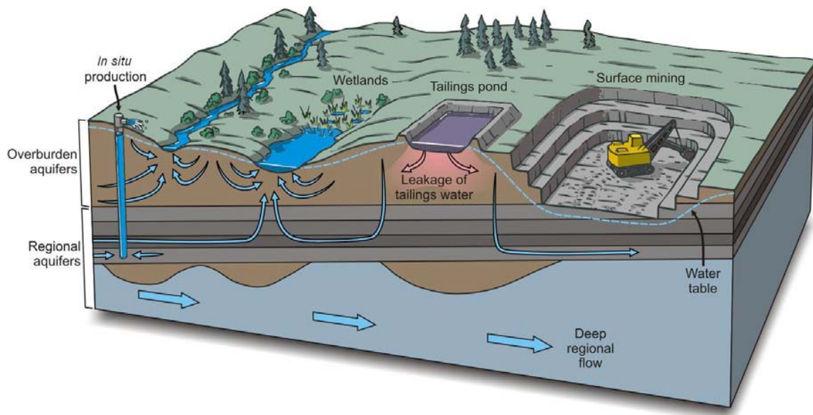
Figure 3-1: Typical Groundwater Flow Patterns in the Vicinity of Oil Sands In-situ and Surface Mining Projects (ARC in CCA 2009)
